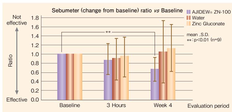
1wt.% AJIDEW® ZN-100 solution exhibits a statistically significant decrease in sebum levels on the treated skin at week 4 compared to baseline.
